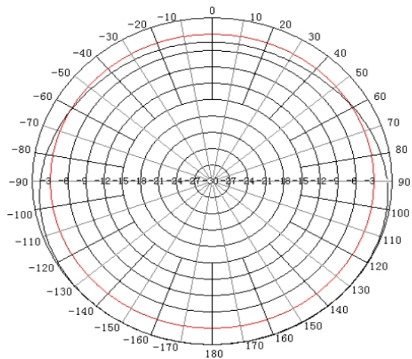
5GHz H Plane
