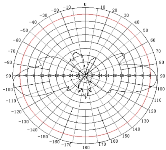
2.4GHz E Plane
