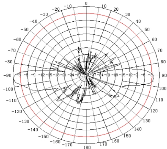
5GHz E Plane
