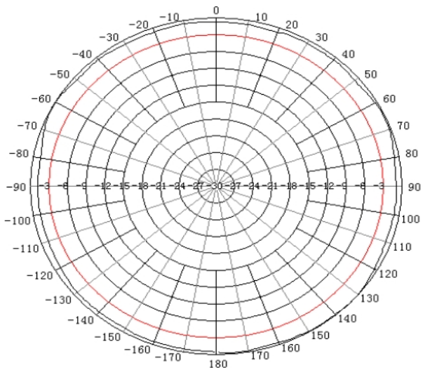
2.4GHz H Plane
