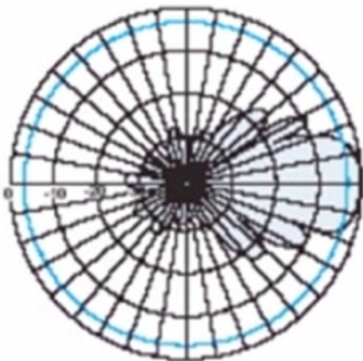
34 degree E plane
