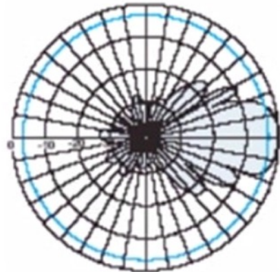
34 degree H plane
